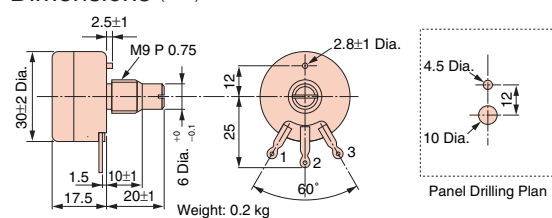
Dimensions (mm)
