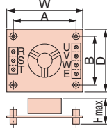
Figure 2 (Three-Phase)
