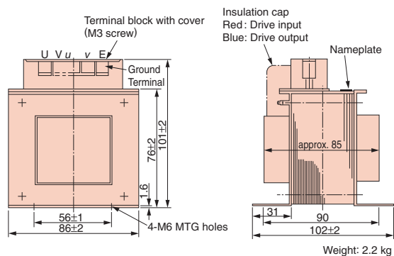
Dimensions (mm)
