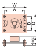
Figure 1 (Single-Phase)
