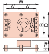
Figure 3 (Three-Phase)
