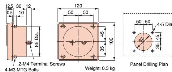
Dimensions (mm)
